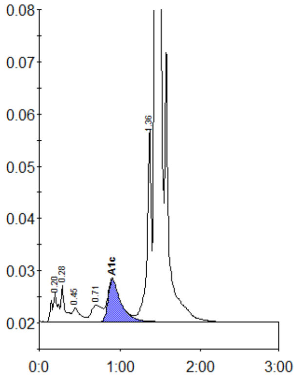
Peak table - ID: 10553216
